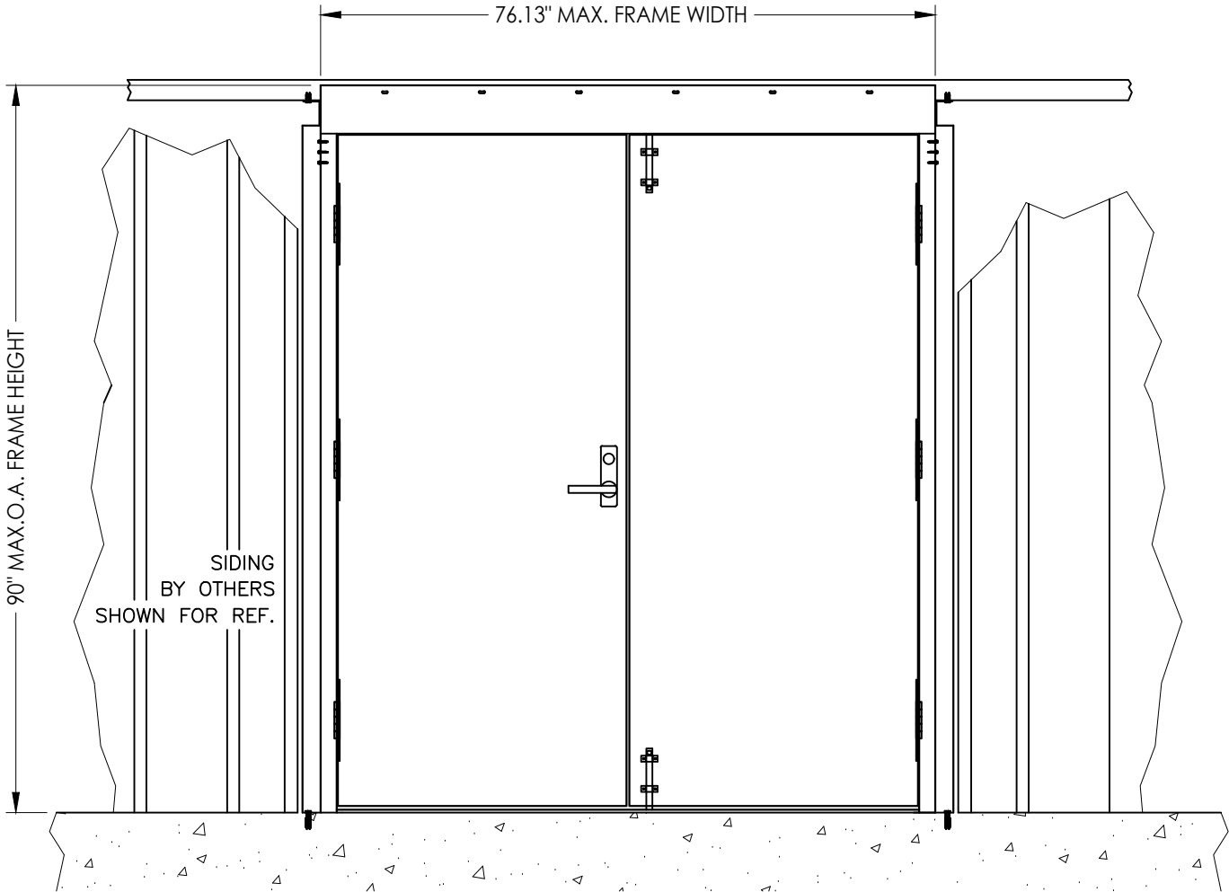
6070 PRE-ASSEMBLED DOOR ELEVATION (Metal building installation)
